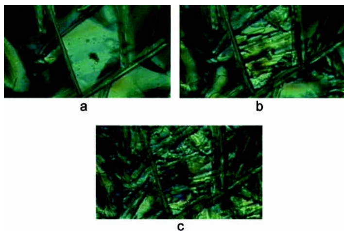
FIGURE 3 Textures of F8H10: a) T = 18.5^{\circ}\text{C} , b) T = -13.2^{\circ}\text{C} , c) T = -47.4^{\circ}\text{C} .
