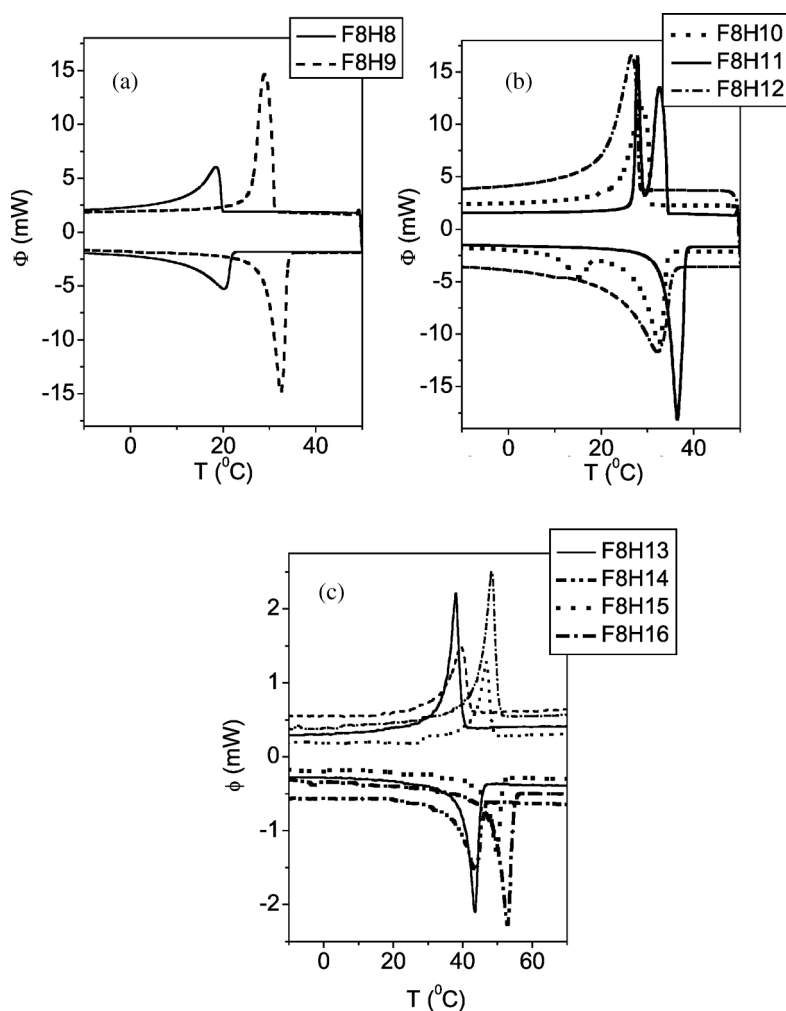
FIGURE 2 DSC curves for the investigated perfluorooctyl- n -alkanes.
