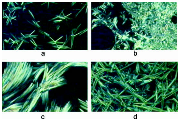
FIGURE 5 Textures of perfluoroisononyl- n -alkanes: a) iF9H7 ( T = -17.3^{\circ}\text{C} ), b) iF9H10 ( T = 13.3^{\circ}\text{C} ), c) iF9H11 ( T = 27.9^{\circ}\text{C} ), d) iF9H15 ( T = 39.1^{\circ}\text{C} ).
