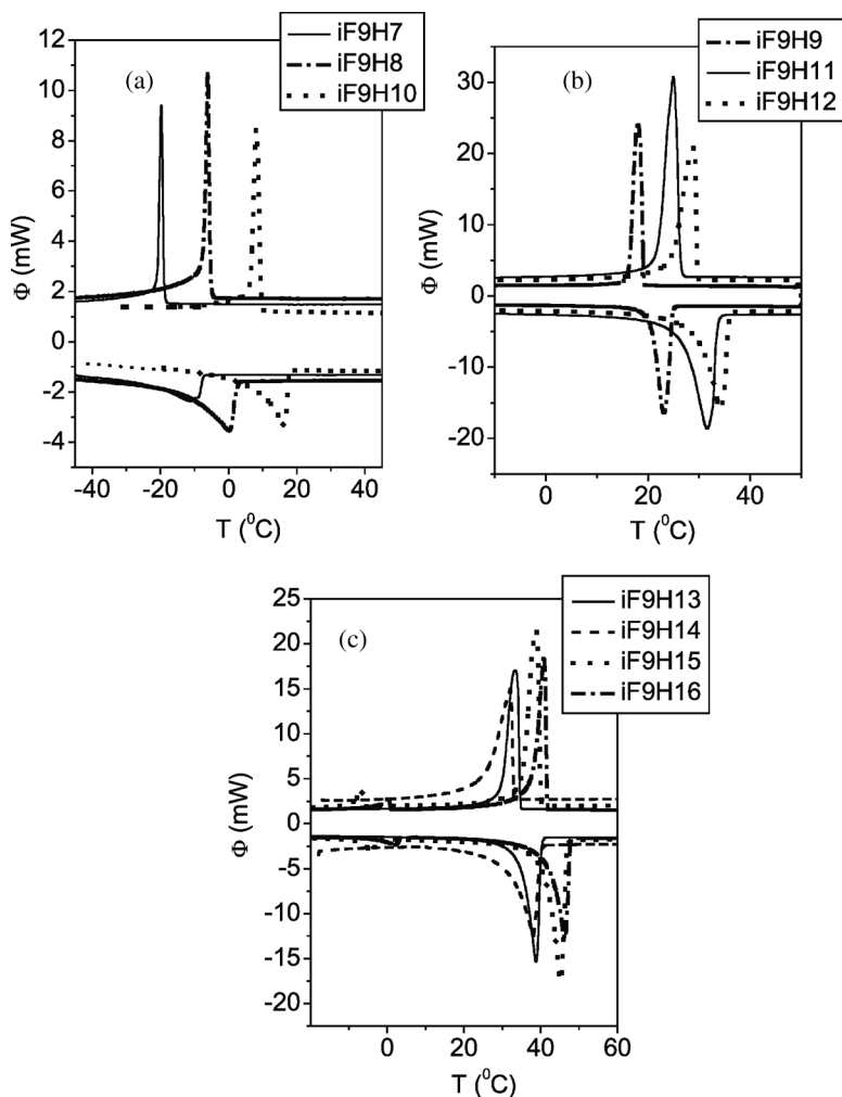
FIGURE 6 DSC curves for the investigated perfluoroisononyl-n-alkanes.
