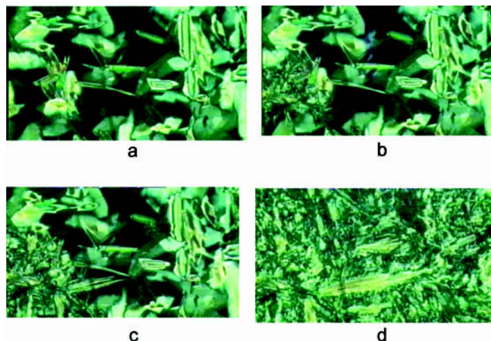
FIGURE 4 Textures of F8H11: a) T=32.9^{\circ}\text{C} , b) T=28.8^{\circ}\text{C} , c) T=28.7^{\circ}\text{C} , d) T=28.3^{\circ}\text{C} ; heating rate: 0.2^{\circ}\text{min}^{-1} .
